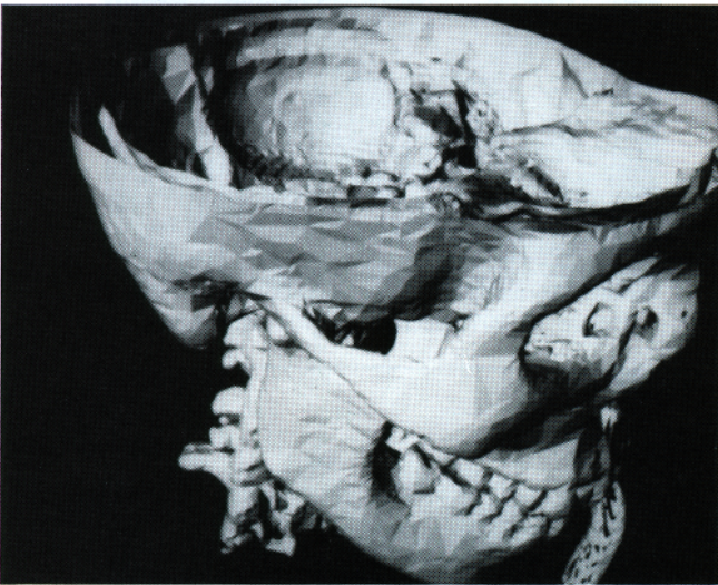
Figure 5c. 75% decimated (142k flat shaded triangles).
