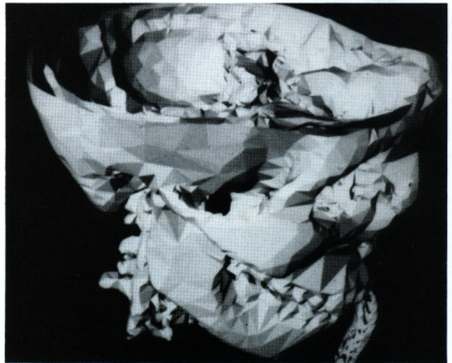
Figure 5d. 90% decimated (57k flat shaded triangles).
