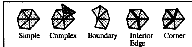
Figure 1. Vertex classifications.
