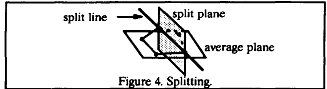
Figure 4. Splitting.
